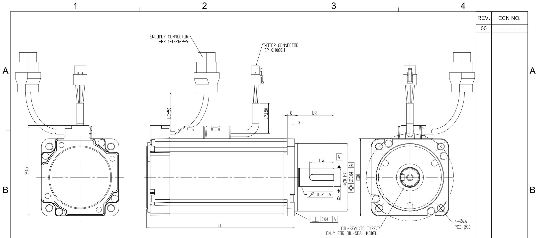
DIMENSION TABLE(MODEL WITH BRAKE)
