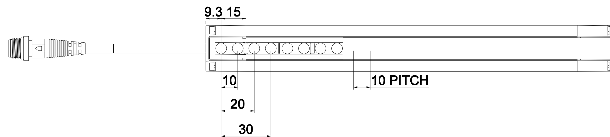
AS-BH□□□ series Pitch:20mm
